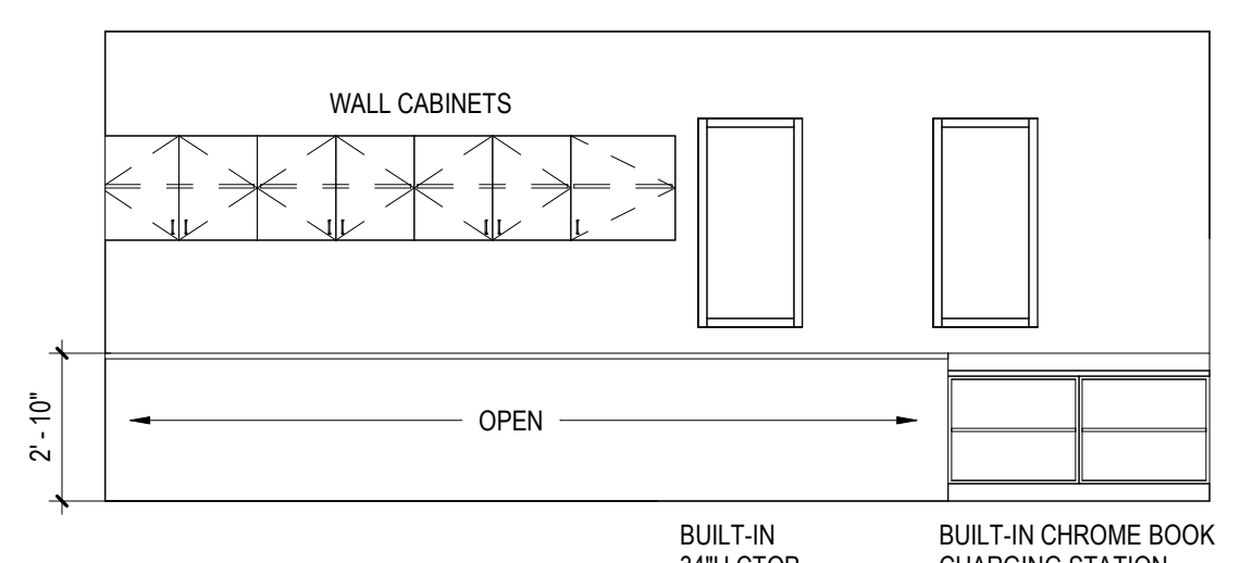
B INTERIOR ELEVATION B 14.2 1/4" = 1'-0"
