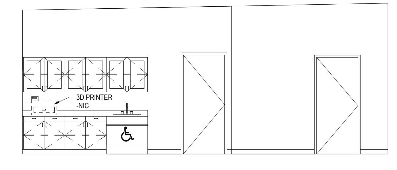
D INTERIOR ELEVATION D 14.2 1/4" = 1'-0"
