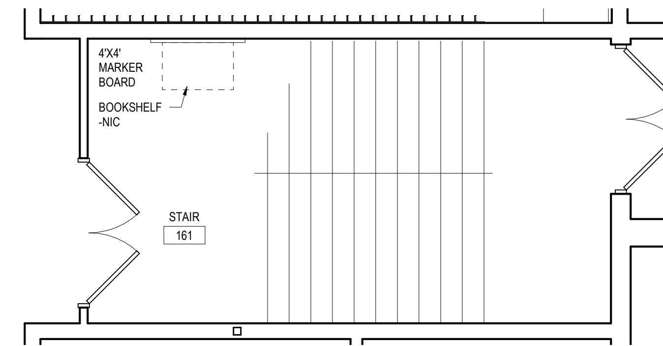
3 STAIR TYP 14.6 1/4" = 1'-0"
