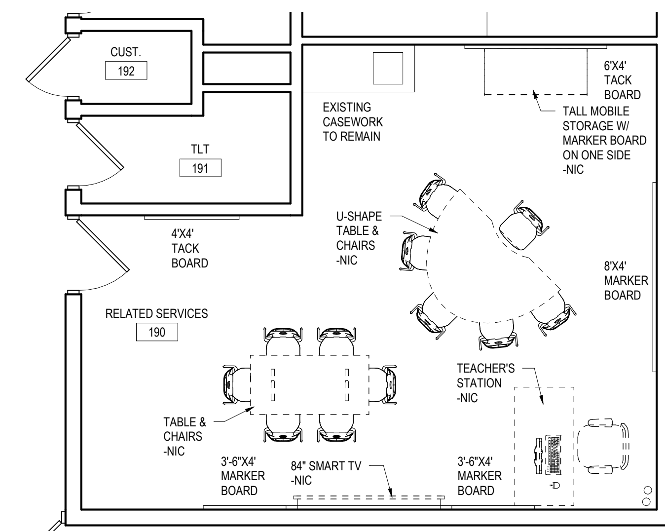
4 RELATED SERVICES 14.6 1/4" = 1'-0"
