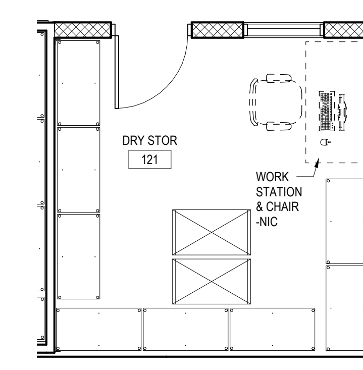
5 KITCHEN OFFICE 14.6 1/4" = 1'-0"
