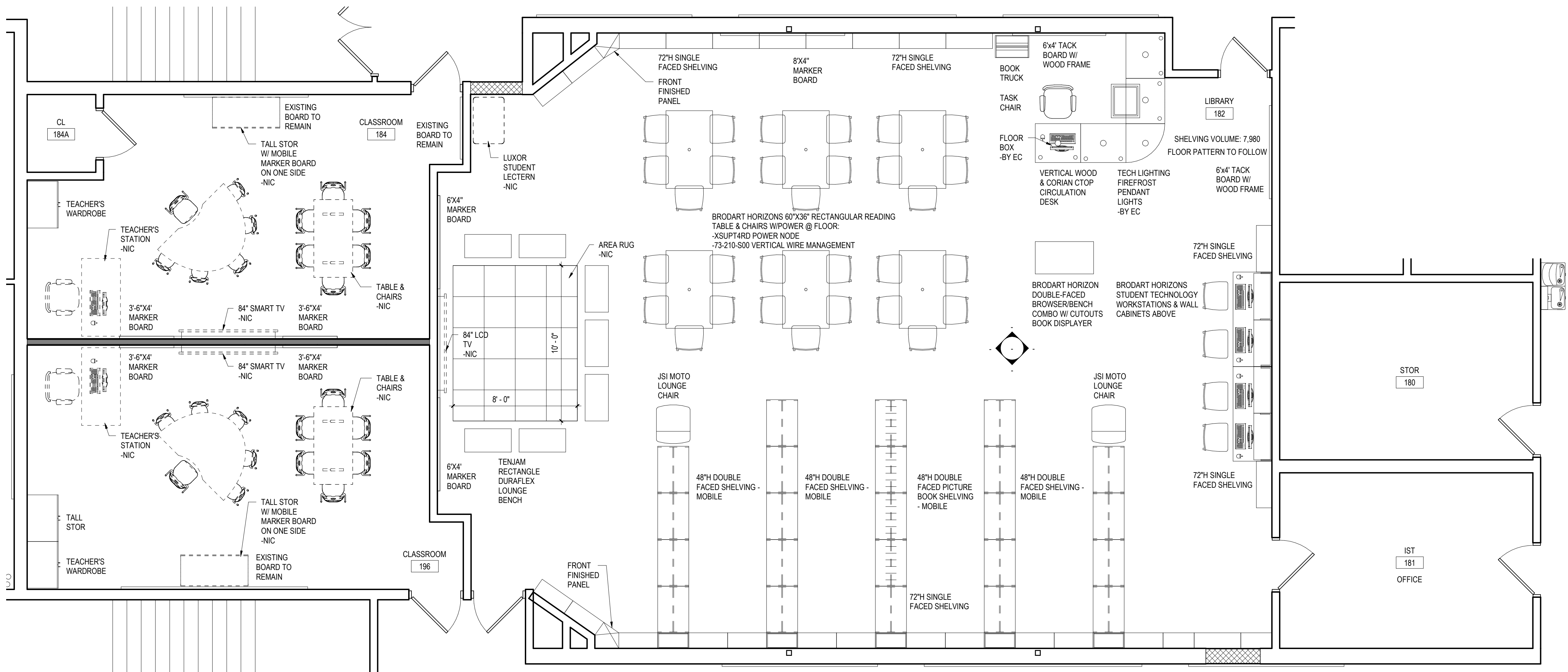
1 LIBRARY & CLASSROOMS 1/4" = 1'-0"
